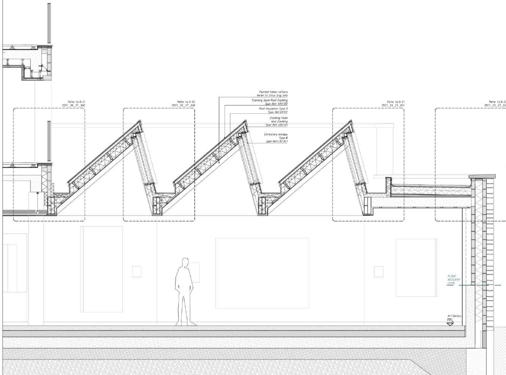
D-01 Section through Sawtooth Roof
