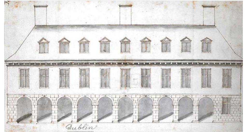
Elevation of William Robinson's new building for the southeast range of Dublin Castle c. 1684
