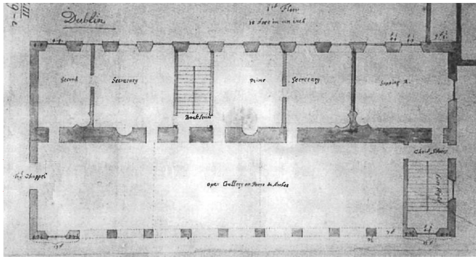
Ground Floor Plan of Robinson Block, 1680s
