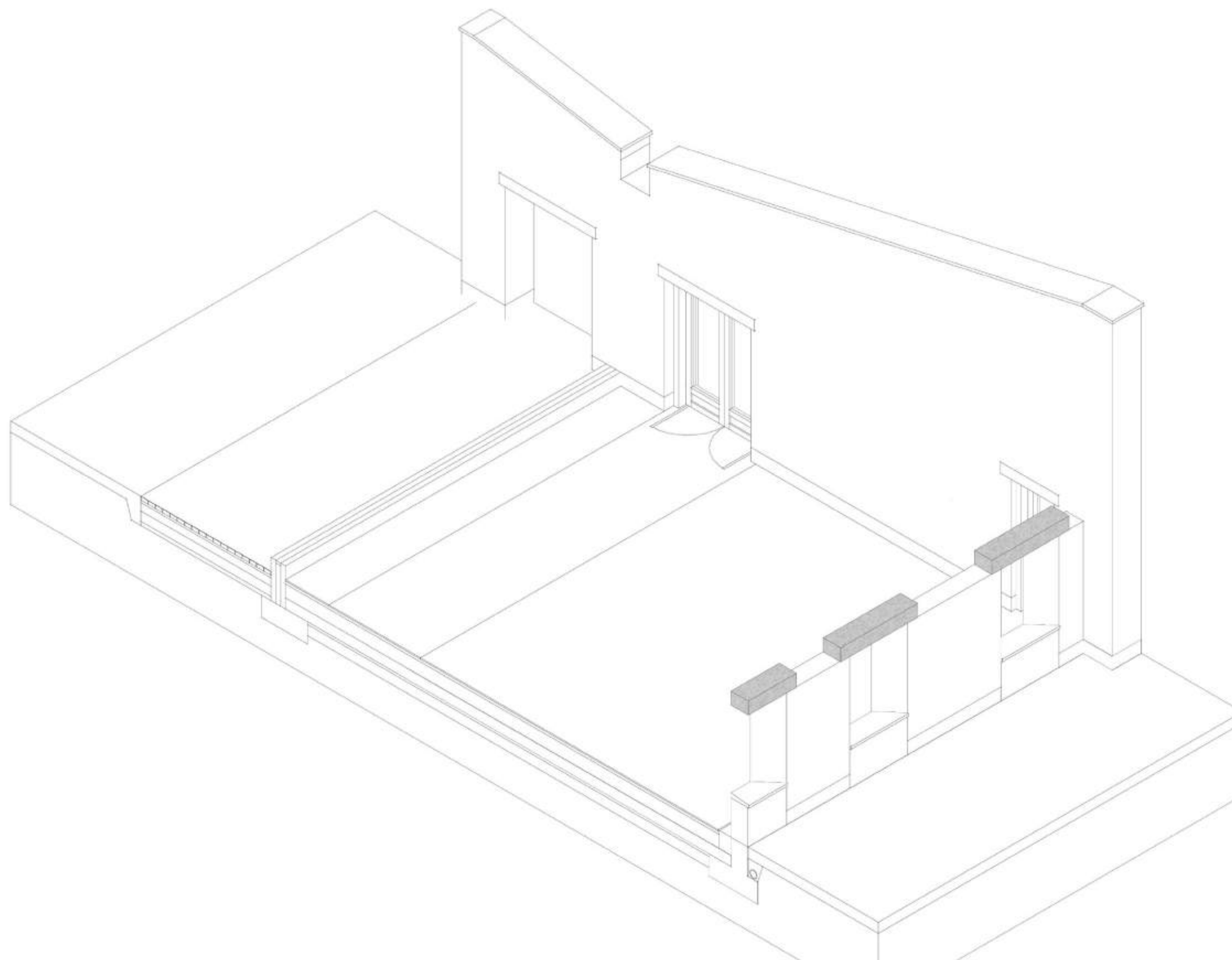
Wall Construction Sequence
