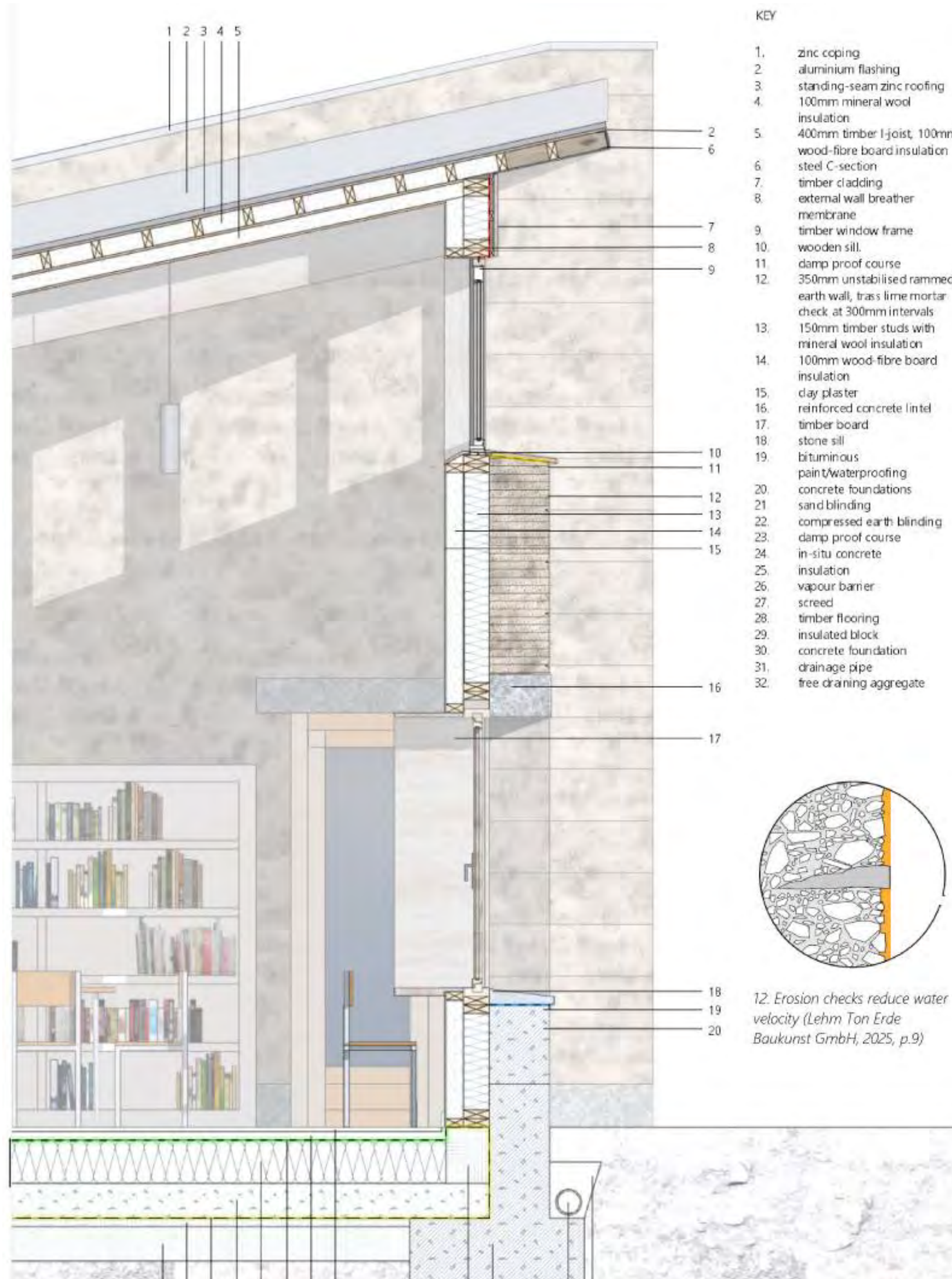
Creating a Rammed Earth Facade
